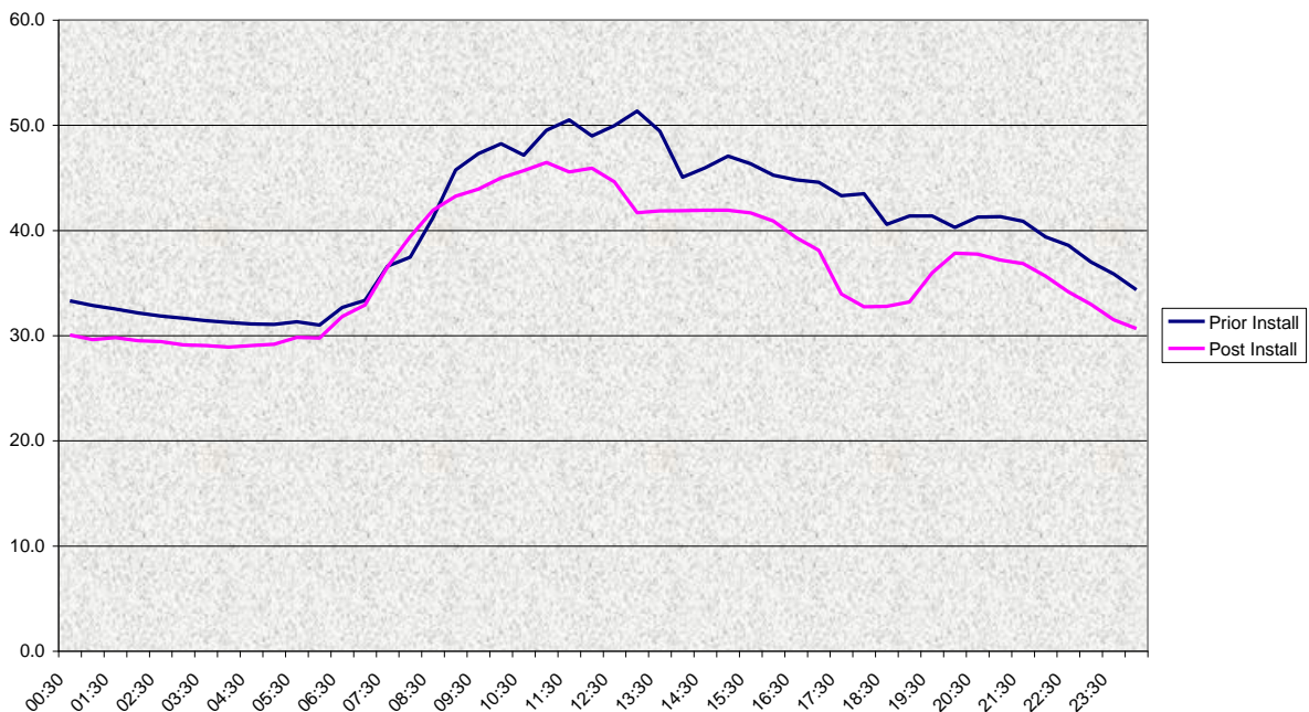
Rathbone 28 Day HHD Comparison Pre & Post Installation
